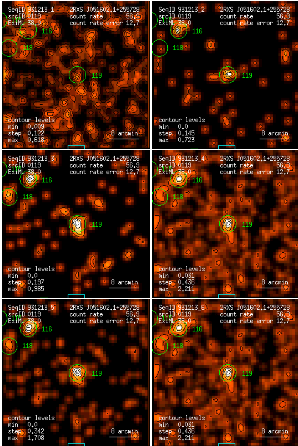
Figure 119: RASS 931213: detection 0119: band rate images, Gaussian filter: (1) PSPC channels 11 – 41, (2) 52 – 90, (3) 91 – 201, (4) 11 – 235, (5) 52 – 201, (6) 11 – 201. Broad band rates in counts/ks. Band rate contour levels in counts/ks/arcmin 2 .
