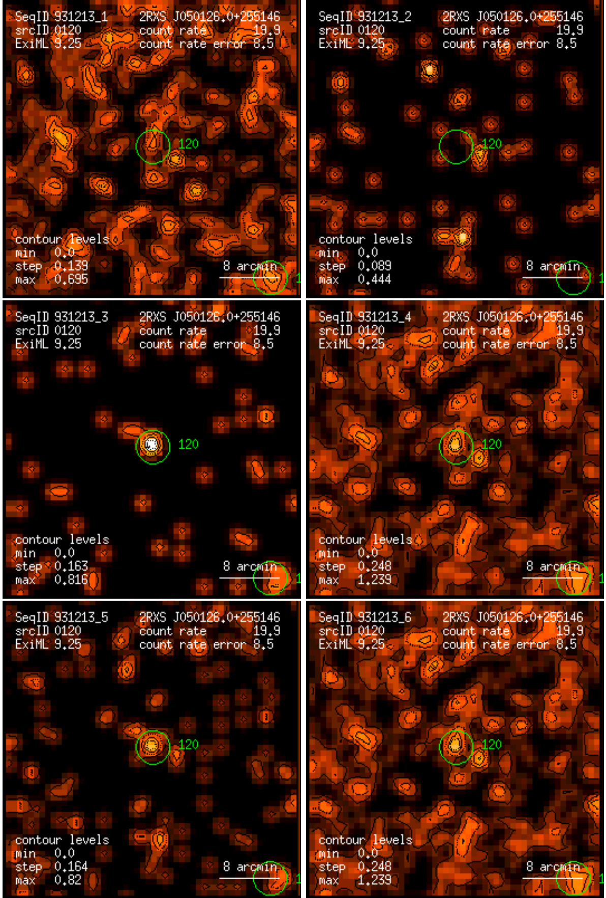
Figure 120: RASS 931213: detection 0120: band rate images, Gaussian filter: (1) PSPC channels 11 – 41, (2) 52 – 90, (3) 91 – 201, (4) 11 – 235, (5) 52 – 201, (6) 11 – 201. Broad band rates in counts/ks. Band rate contour levels in counts/ks/arcmin 2 .
