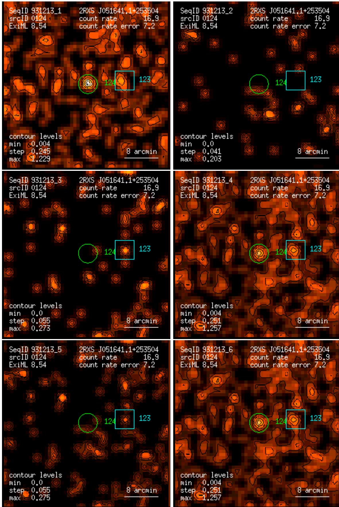
Figure 124: RASS 931213: detection 0124: band rate images, Gaussian filter: (1) PSPC channels 11 – 41, (2) 52 – 90, (3) 91 – 201, (4) 11 – 235, (5) 52 – 201, (6) 11 – 201. Broad band rates in counts/ks. Band rate contour levels in counts/ks/arcmin 2 .
