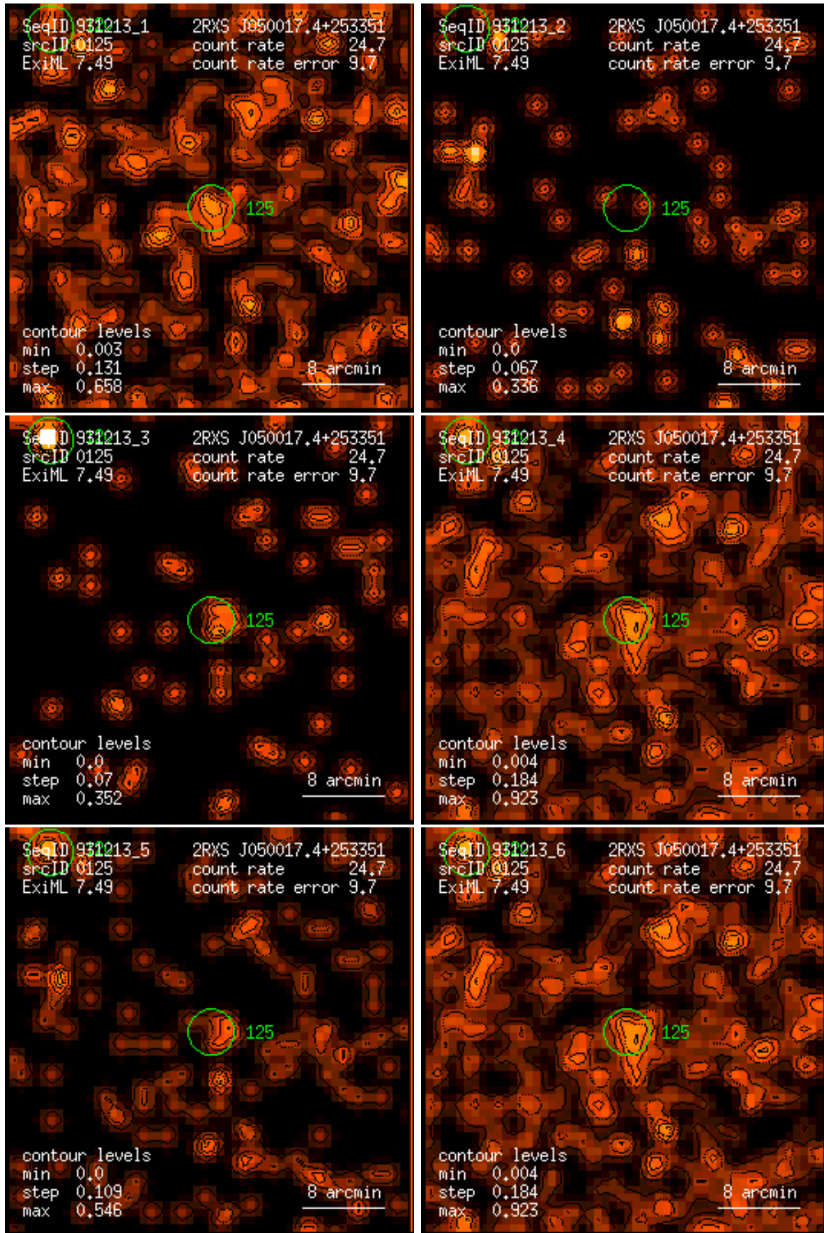
Figure 125: RASS 931213: detection 0125: band rate images, Gaussian filter: (1) PSPC channels 11 – 41, (2) 52 – 90, (3) 91 – 201, (4) 11 – 235, (5) 52 – 201, (6) 11 – 201. Broad band rates in counts/ks. Band rate contour levels in counts/ks/arcmin 2 .
