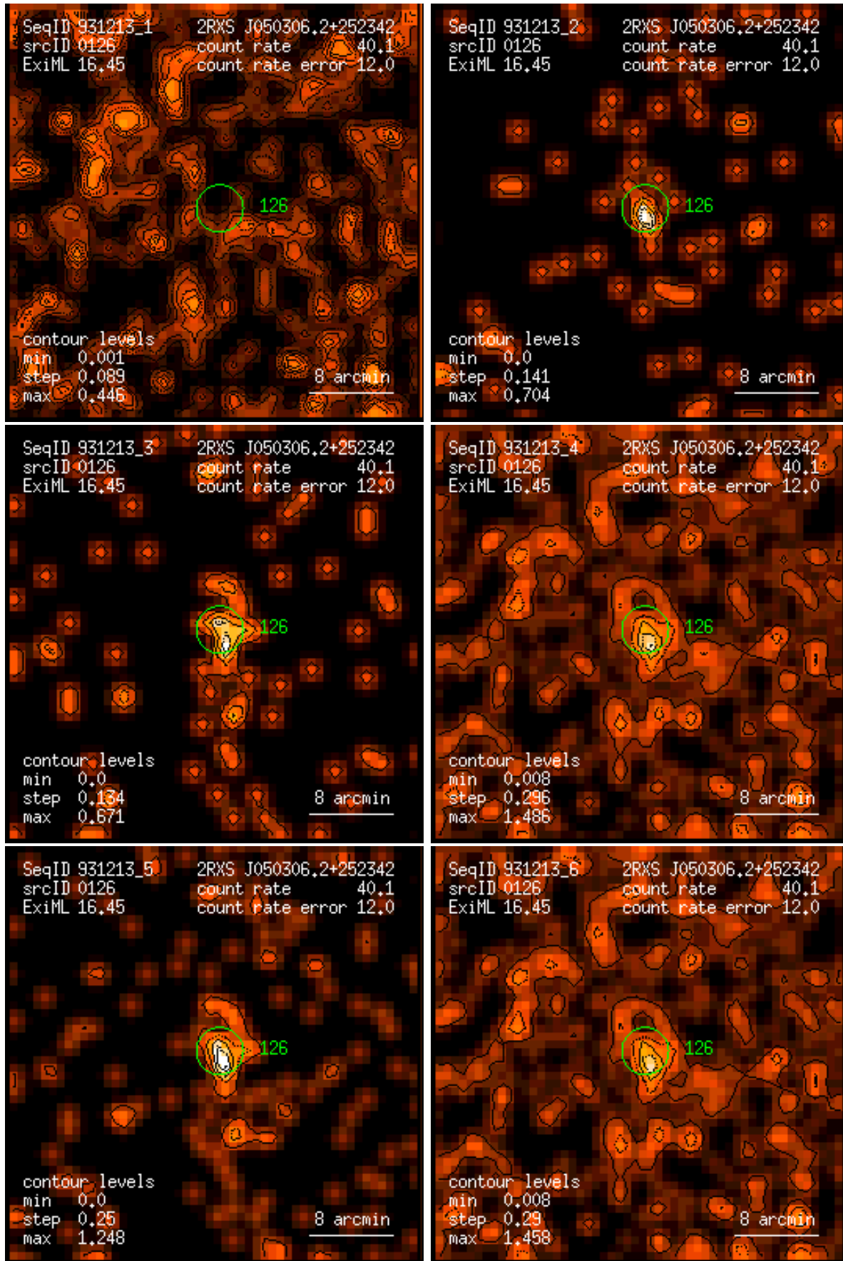
Figure 126: RASS 931213: detection 0126: band rate images, Gaussian filter: (1) PSPC channels 11 – 41, (2) 52 – 90, (3) 91 – 201, (4) 11 – 235, (5) 52 – 201, (6) 11 – 201. Broad band rates in counts/ks. Band rate contour levels in counts/ks/arcmin 2 .
