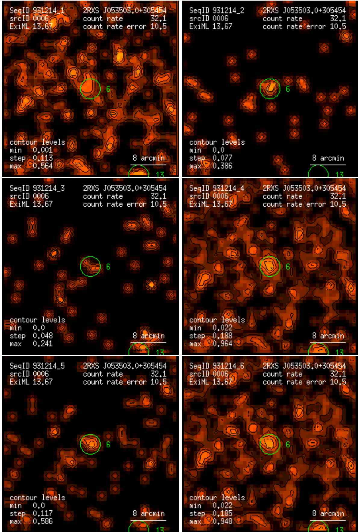
Figure 6: RASS 931214: detection 0006: band rate images, Gaussian filter: (1) PSPC channels 11 – 41, (2) 52 – 90, (3) 91 – 201, (4) 11 – 235, (5) 52 – 201, (6) 11 – 201. Broad band rates in counts/ks. Band rate contour levels in counts/ks/arcmin 2 .
