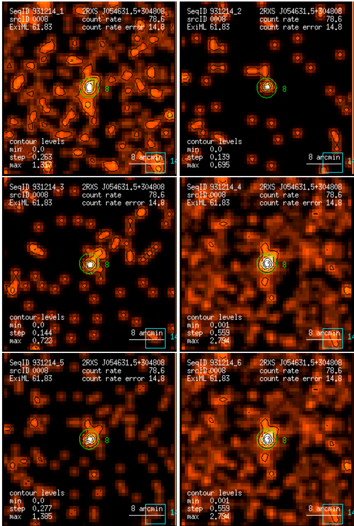
Figure 8: RASS 931214: detection 0008: band rate images, Gaussian filter: (1) PSPC channels 11 – 41, (2) 52 – 90, (3) 91 – 201, (4) 11 – 235, (5) 52 – 201, (6) 11 – 201. Broad band rates in counts/ks. Band rate contour levels in counts/ks/arcmin 2 .
