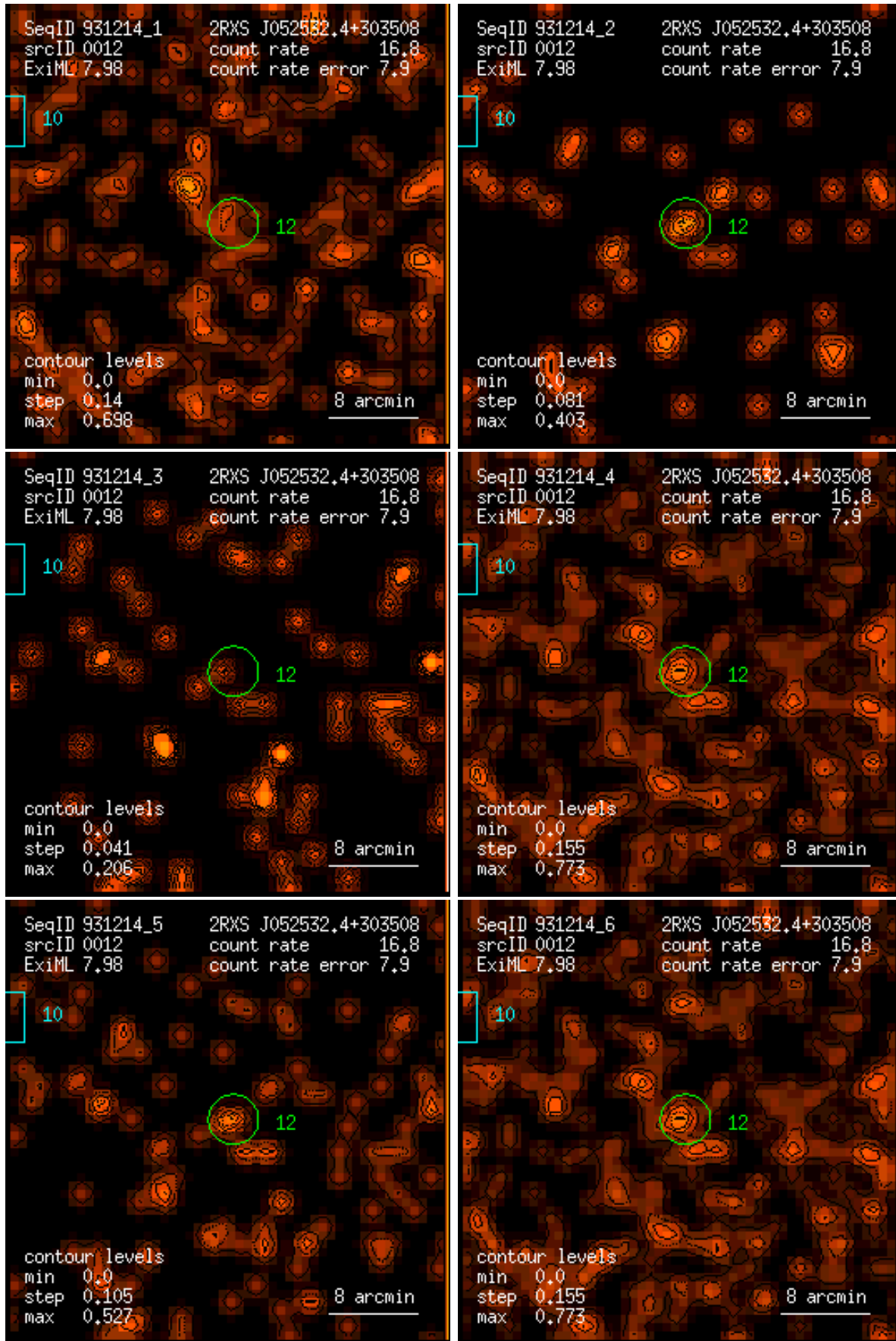
Figure 12: RASS 931214: detection 0012: band rate images, Gaussian filter: (1) PSPC channels 11 – 41, (2) 52 – 90, (3) 91 – 201, (4) 11 – 235, (5) 52 – 201, (6) 11 – 201. Broad band rates in counts/ks. Band rate contour levels in counts/ks/arcmin 2 .
