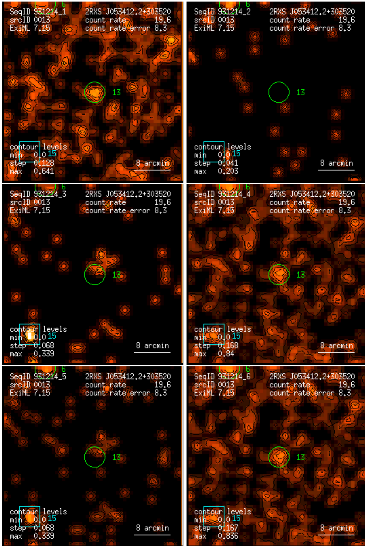
Figure 13: RASS 931214: detection 0013: band rate images, Gaussian filter: (1) PSPC channels 11 – 41, (2) 52 – 90, (3) 91 – 201, (4) 11 – 235, (5) 52 – 201, (6) 11 – 201. Broad band rates in counts/ks. Band rate contour levels in counts/ks/arcmin 2 .
