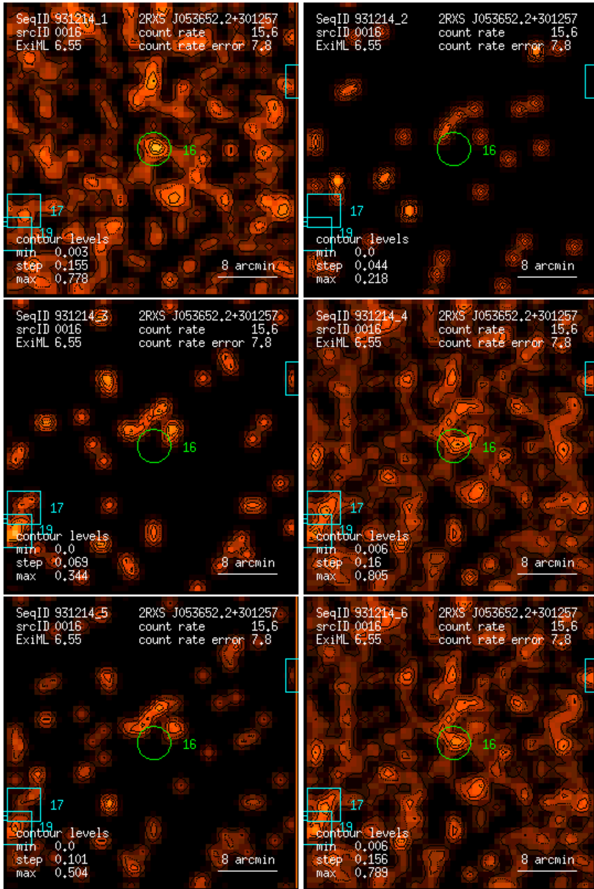
Figure 16: RASS 931214: detection 0016: band rate images, Gaussian filter: (1) PSPC channels 11 – 41, (2) 52 – 90, (3) 91 – 201, (4) 11 – 235, (5) 52 – 201, (6) 11 – 201. Broad band rates in counts/ks. Band rate contour levels in counts/ks/arcmin 2 .
