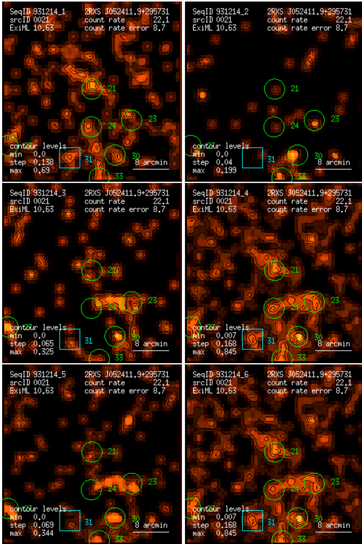
Figure 21: RASS 931214: detection 0021: band rate images, Gaussian filter: (1) PSPC channels 11 – 41, (2) 52 – 90, (3) 91 – 201, (4) 11 – 235, (5) 52 – 201, (6) 11 – 201. Broad band rates in counts/ks. Band rate contour levels in counts/ks/arcmin 2 .
