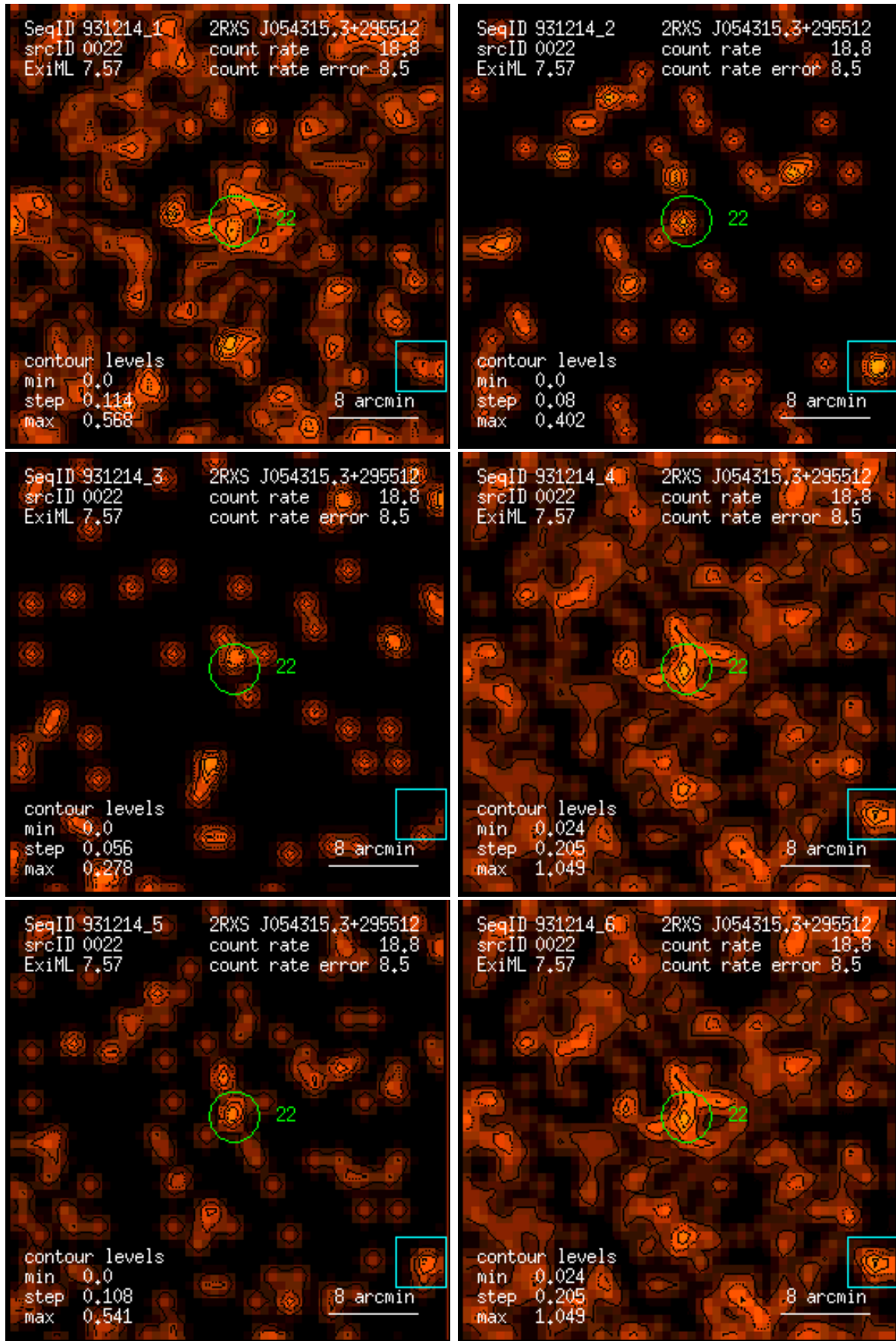
Figure 22: RASS 931214: detection 0022: band rate images, Gaussian filter: (1) PSPC channels 11 – 41, (2) 52 – 90, (3) 91 – 201, (4) 11 – 235, (5) 52 – 201, (6) 11 – 201. Broad band rates in counts/ks. Band rate contour levels in counts/ks/arcmin 2 .
