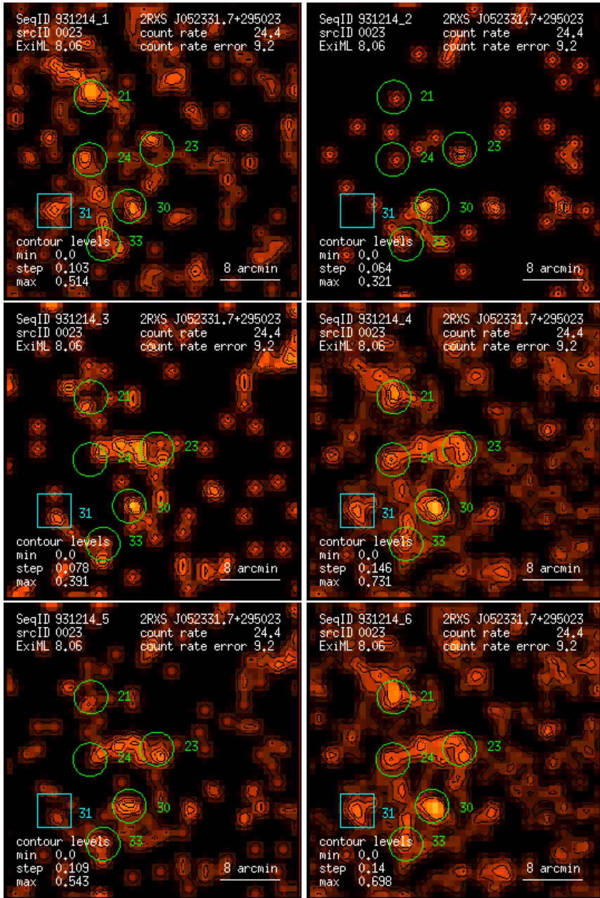
Figure 23: RASS 931214: detection 0023: band rate images, Gaussian filter: (1) PSPC channels 11 – 41, (2) 52 – 90, (3) 91 – 201, (4) 11 – 235, (5) 52 – 201, (6) 11 – 201. Broad band rates in counts/ks. Band rate contour levels in counts/ks/arcmin 2 .
