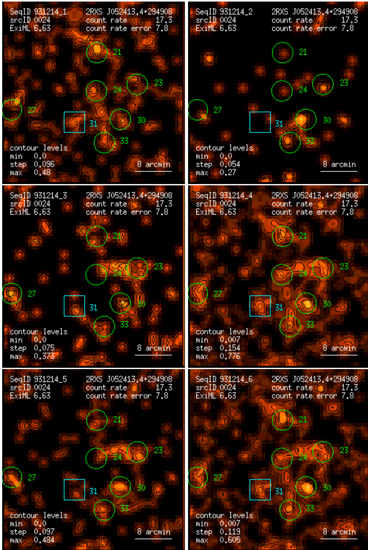
Figure 24: RASS 931214: detection 0024: band rate images, Gaussian filter: (1) PSPC channels 11 – 41, (2) 52 – 90, (3) 91 – 201, (4) 11 – 235, (5) 52 – 201, (6) 11 – 201. Broad band rates in counts/ks. Band rate contour levels in counts/ks/arcmin 2 .
