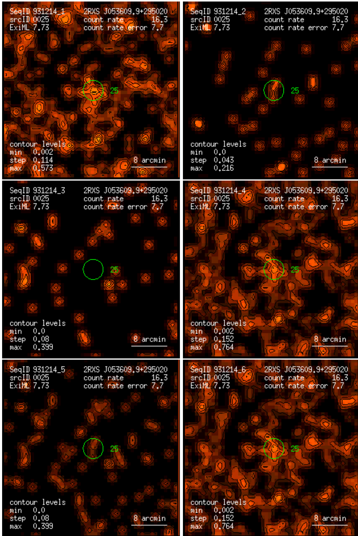
Figure 25: RASS 931214: detection 0025: band rate images, Gaussian filter: (1) PSPC channels 11 – 41, (2) 52 – 90, (3) 91 – 201, (4) 11 – 235, (5) 52 – 201, (6) 11 – 201. Broad band rates in counts/ks. Band rate contour levels in counts/ks/arcmin 2 .
