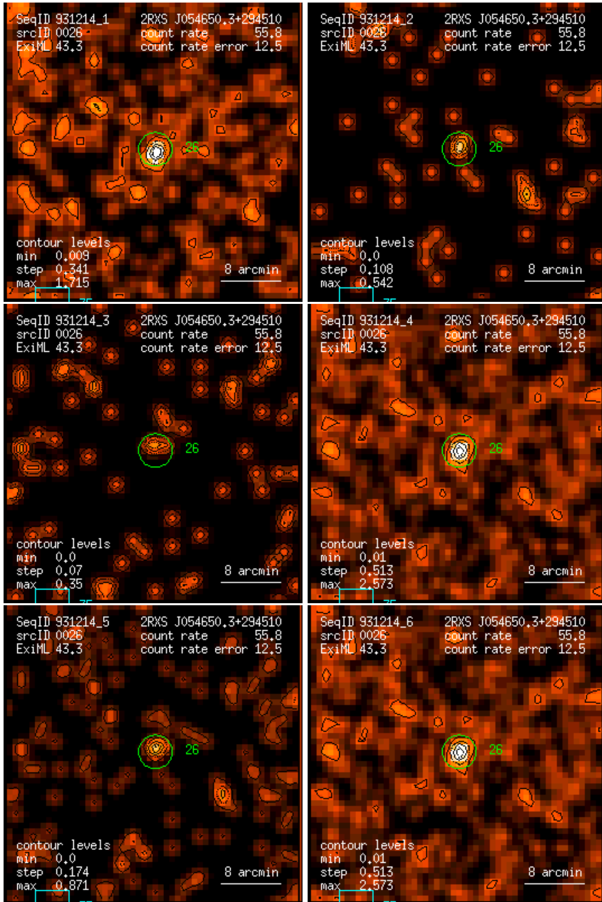
Figure 26: RASS 931214: detection 0026: band rate images, Gaussian filter: (1) PSPC channels 11 – 41, (2) 52 – 90, (3) 91 – 201, (4) 11 – 235, (5) 52 – 201, (6) 11 – 201. Broad band rates in counts/ks. Band rate contour levels in counts/ks/arcmin 2 .
