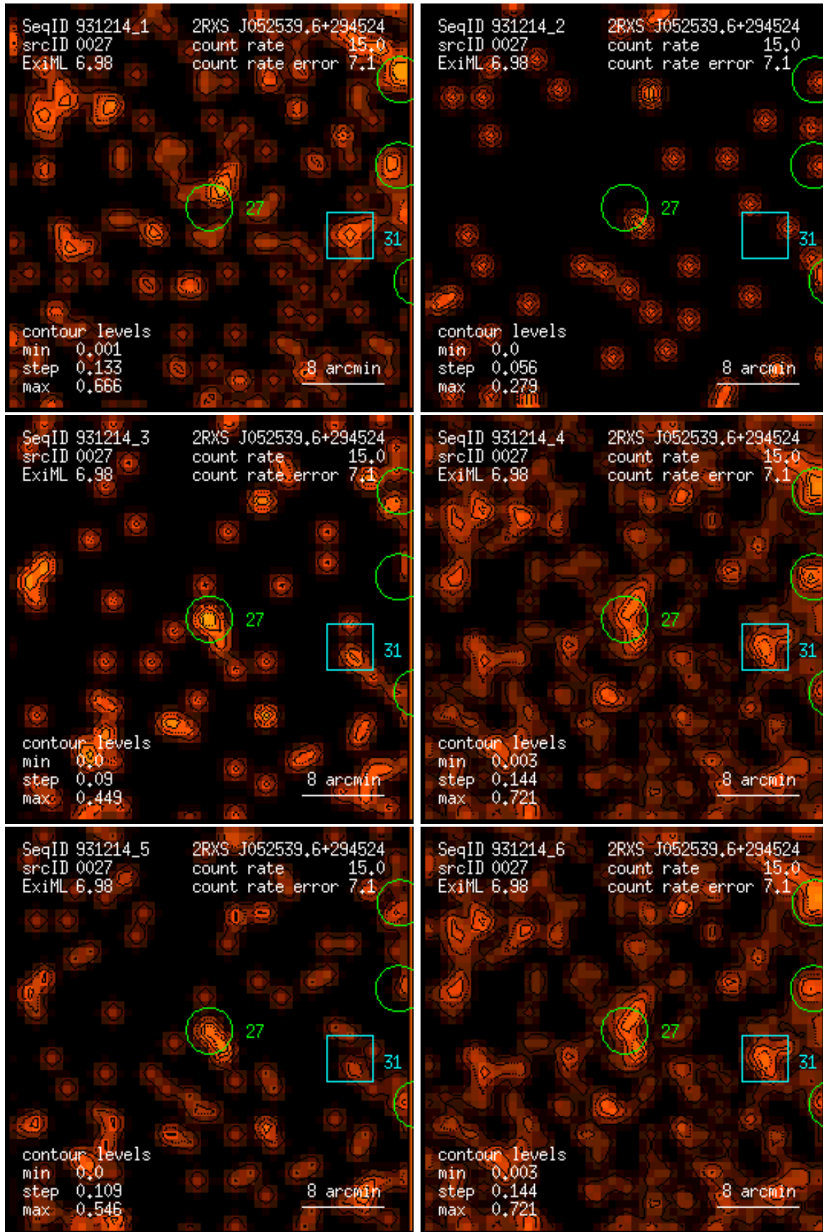
Figure 27: RASS 931214: detection 0027: band rate images, Gaussian filter: (1) PSPC channels 11 – 41, (2) 52 – 90, (3) 91 – 201, (4) 11 – 235, (5) 52 – 201, (6) 11 – 201. Broad band rates in counts/ks. Band rate contour levels in counts/ks/arcmin 2 .
