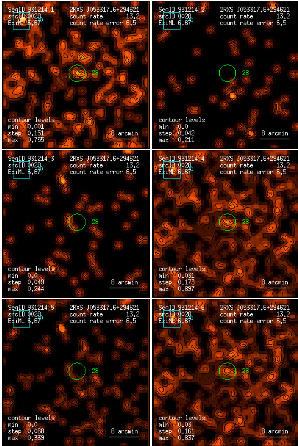
Figure 28: RASS 931214: detection 0028: band rate images, Gaussian filter: (1) PSPC channels 11 – 41, (2) 52 – 90, (3) 91 – 201, (4) 11 – 235, (5) 52 – 201, (6) 11 – 201. Broad band rates in counts/ks. Band rate contour levels in counts/ks/arcmin 2 .
