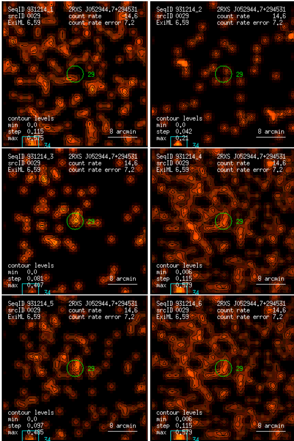
Figure 29: RASS 931214: detection 0029: band rate images, Gaussian filter: (1) PSPC channels 11 – 41, (2) 52 – 90, (3) 91 – 201, (4) 11 – 235, (5) 52 – 201, (6) 11 – 201. Broad band rates in counts/ks. Band rate contour levels in counts/ks/arcmin 2 .
