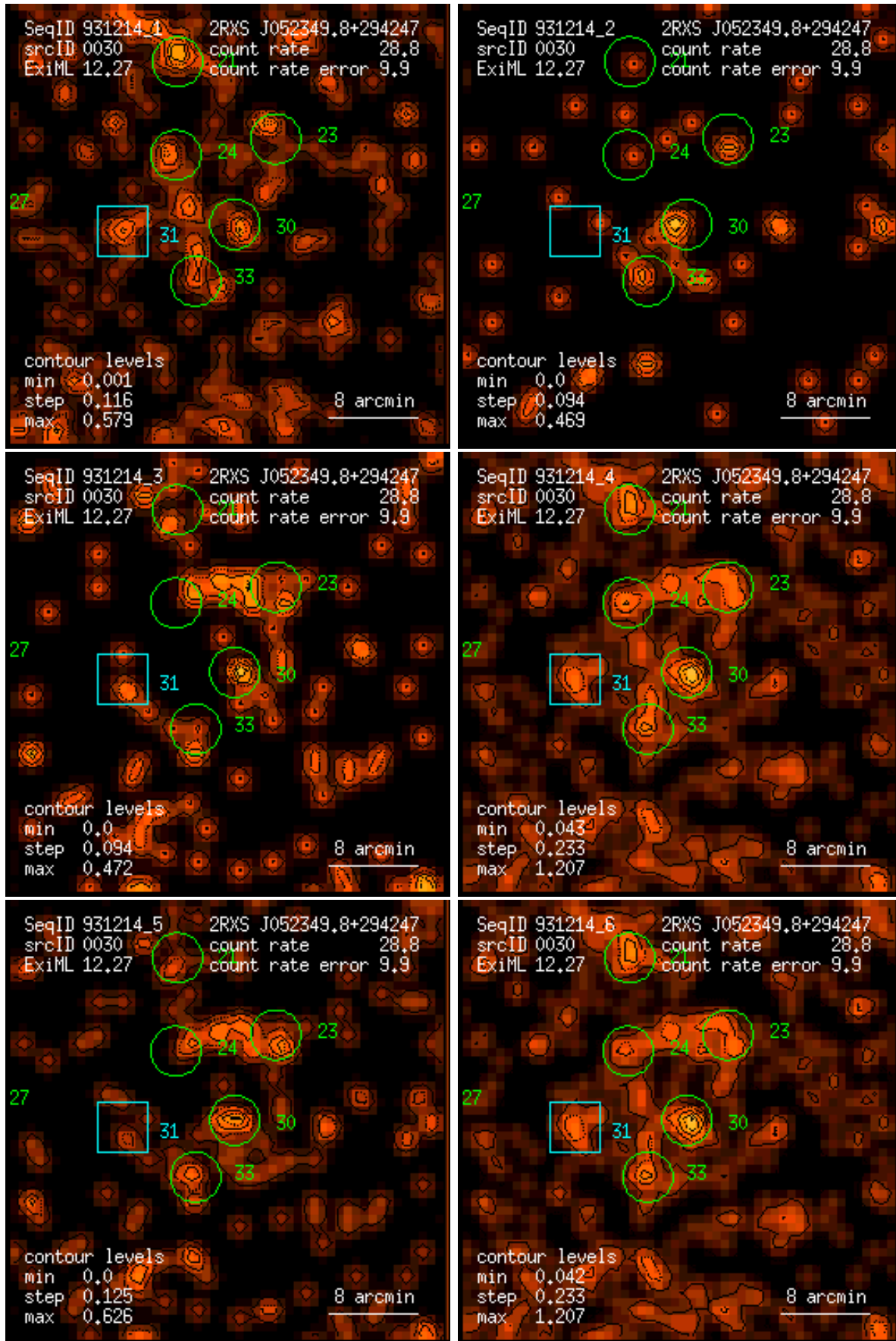
Figure 30: RASS 931214: detection 0030: band rate images, Gaussian filter: (1) PSPC channels 11 – 41, (2) 52 – 90, (3) 91 – 201, (4) 11 – 235, (5) 52 – 201, (6) 11 – 201. Broad band rates in counts/ks. Band rate contour levels in counts/ks/arcmin 2 .
