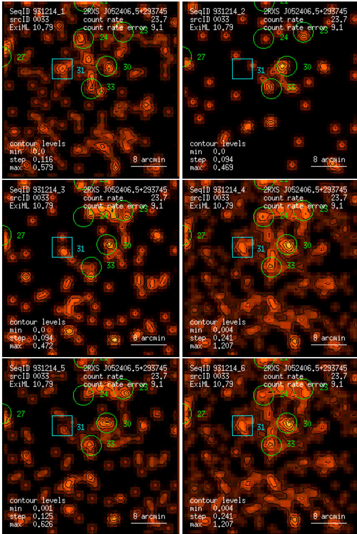
Figure 33: RASS 931214: detection 0033: band rate images, Gaussian filter: (1) PSPC channels 11 – 41, (2) 52 – 90, (3) 91 – 201, (4) 11 – 235, (5) 52 – 201, (6) 11 – 201. Broad band rates in counts/ks. Band rate contour levels in counts/ks/arcmin 2 .
