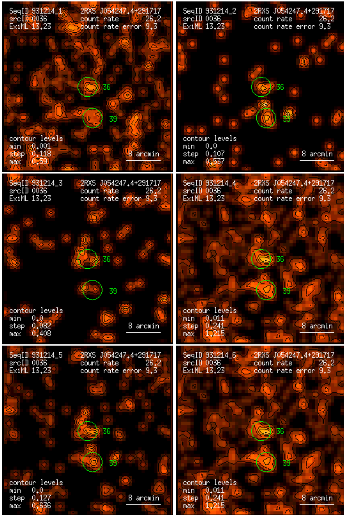
Figure 36: RASS 931214: detection 0036: band rate images, Gaussian filter: (1) PSPC channels 11 – 41, (2) 52 – 90, (3) 91 – 201, (4) 11 – 235, (5) 52 – 201, (6) 11 – 201. Broad band rates in counts/ks. Band rate contour levels in counts/ks/arcmin 2 .
