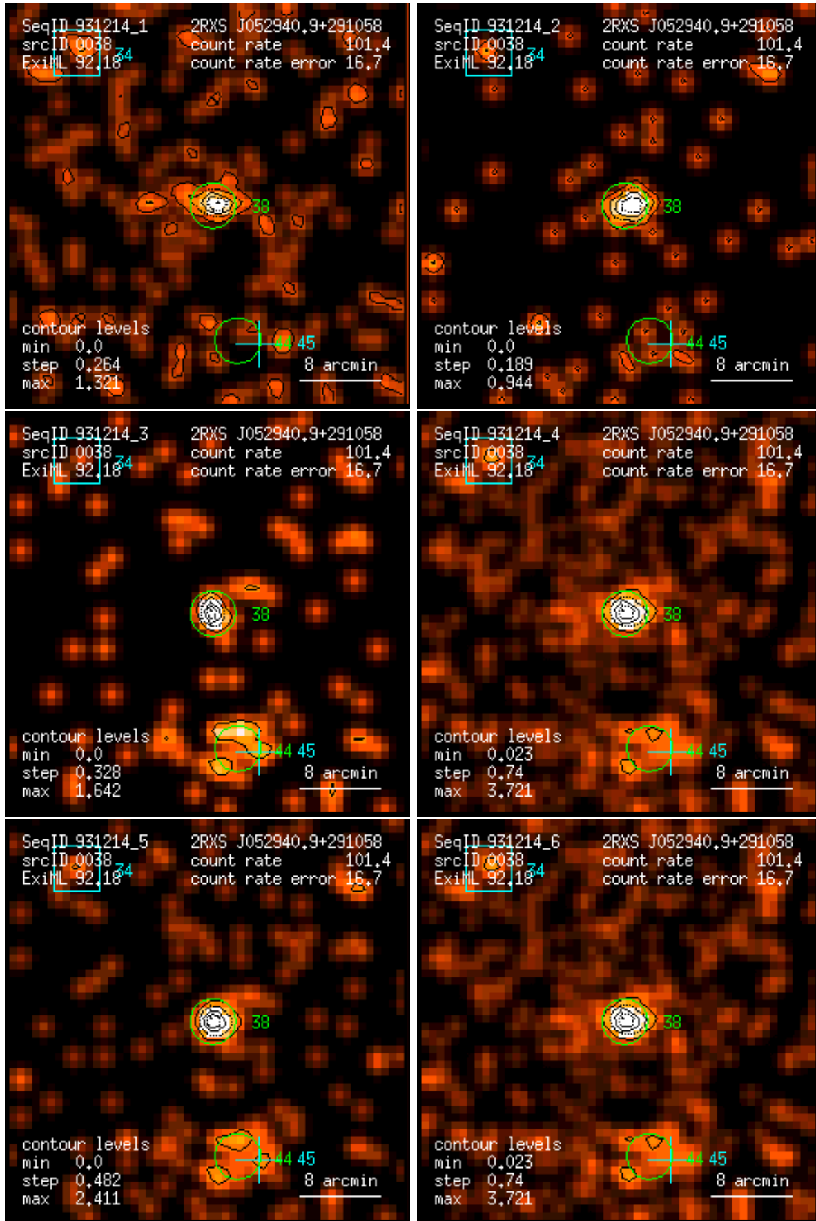
Figure 38: RASS 931214: detection 0038: band rate images, Gaussian filter: (1) PSPC channels 11 – 41, (2) 52 – 90, (3) 91 – 201, (4) 11 – 235, (5) 52 – 201, (6) 11 – 201. Broad band rates in counts/ks. Band rate contour levels in counts/ks/arcmin 2 .
