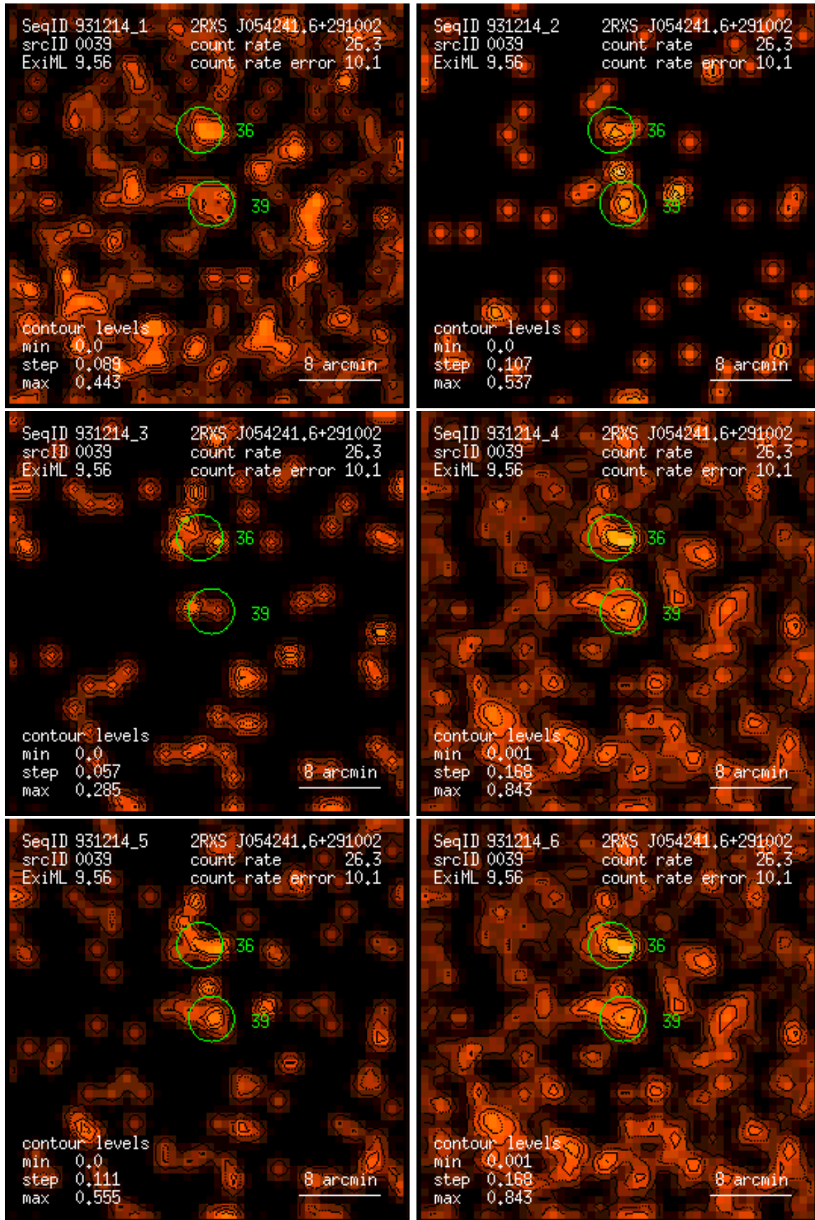
Figure 39: RASS 931214: detection 0039: band rate images, Gaussian filter: (1) PSPC channels 11 – 41, (2) 52 – 90, (3) 91 – 201, (4) 11 – 235, (5) 52 – 201, (6) 11 – 201. Broad band rates in counts/ks. Band rate contour levels in counts/ks/arcmin 2 .
