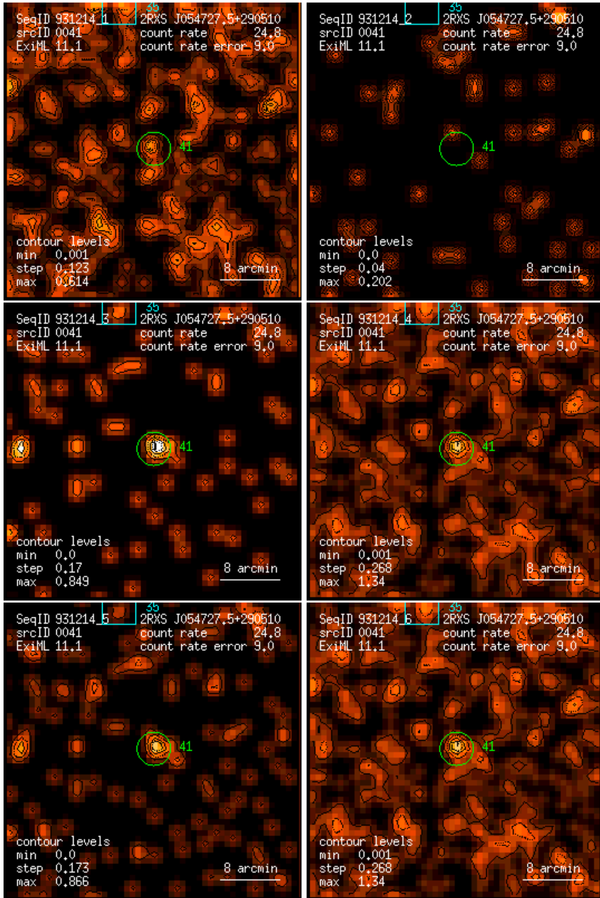
Figure 41: RASS 931214: detection 0041: band rate images, Gaussian filter: (1) PSPC channels 11 – 41, (2) 52 – 90, (3) 91 – 201, (4) 11 – 235, (5) 52 – 201, (6) 11 – 201. Broad band rates in counts/ks. Band rate contour levels in counts/ks/arcmin 2 .
