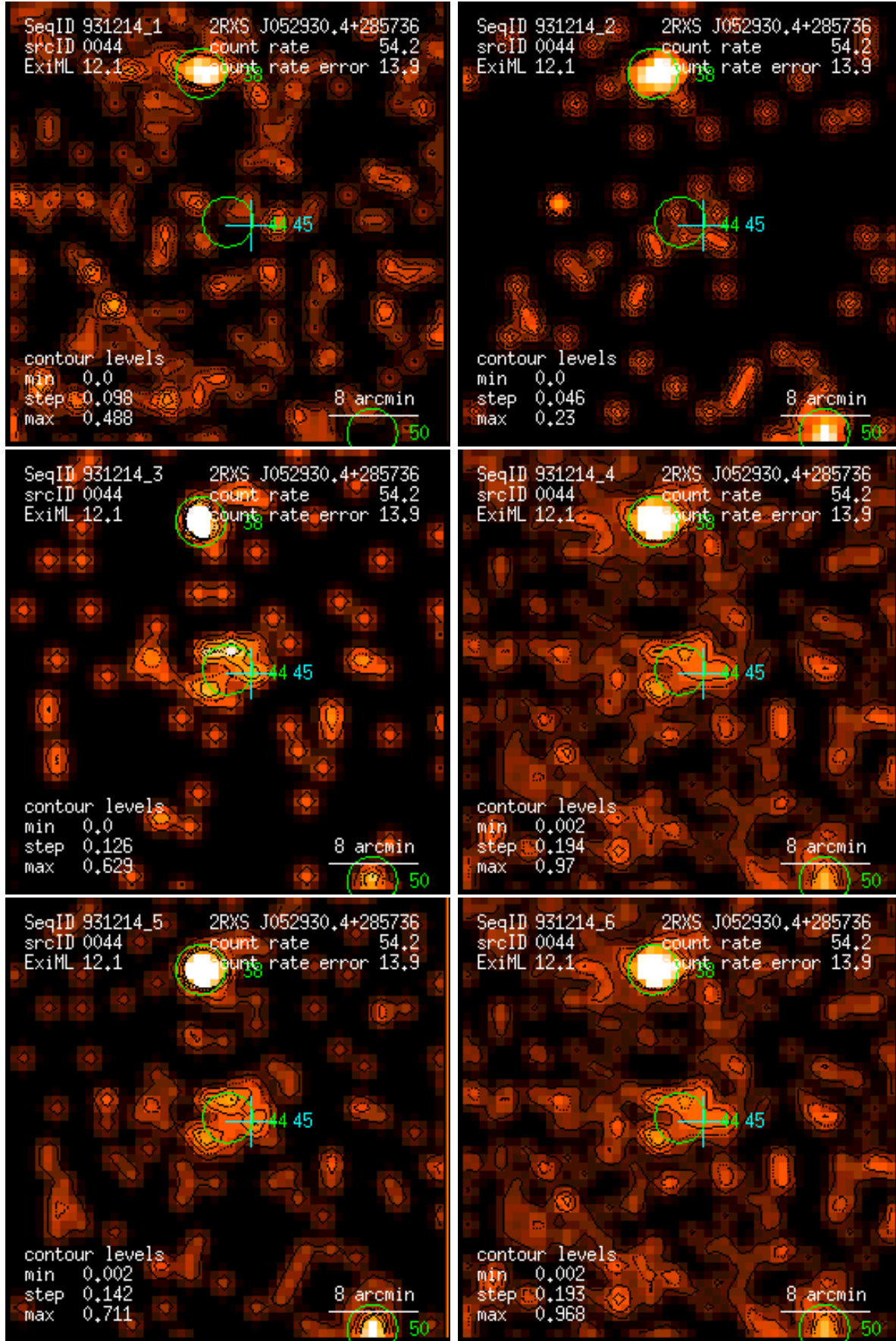
Figure 44: RASS 931214: detection 0044: band rate images, Gaussian filter: (1) PSPC channels 11 – 41, (2) 52 – 90, (3) 91 – 201, (4) 11 – 235, (5) 52 – 201, (6) 11 – 201. Broad band rates in counts/ks. Band rate contour levels in counts/ks/arcmin 2 .
