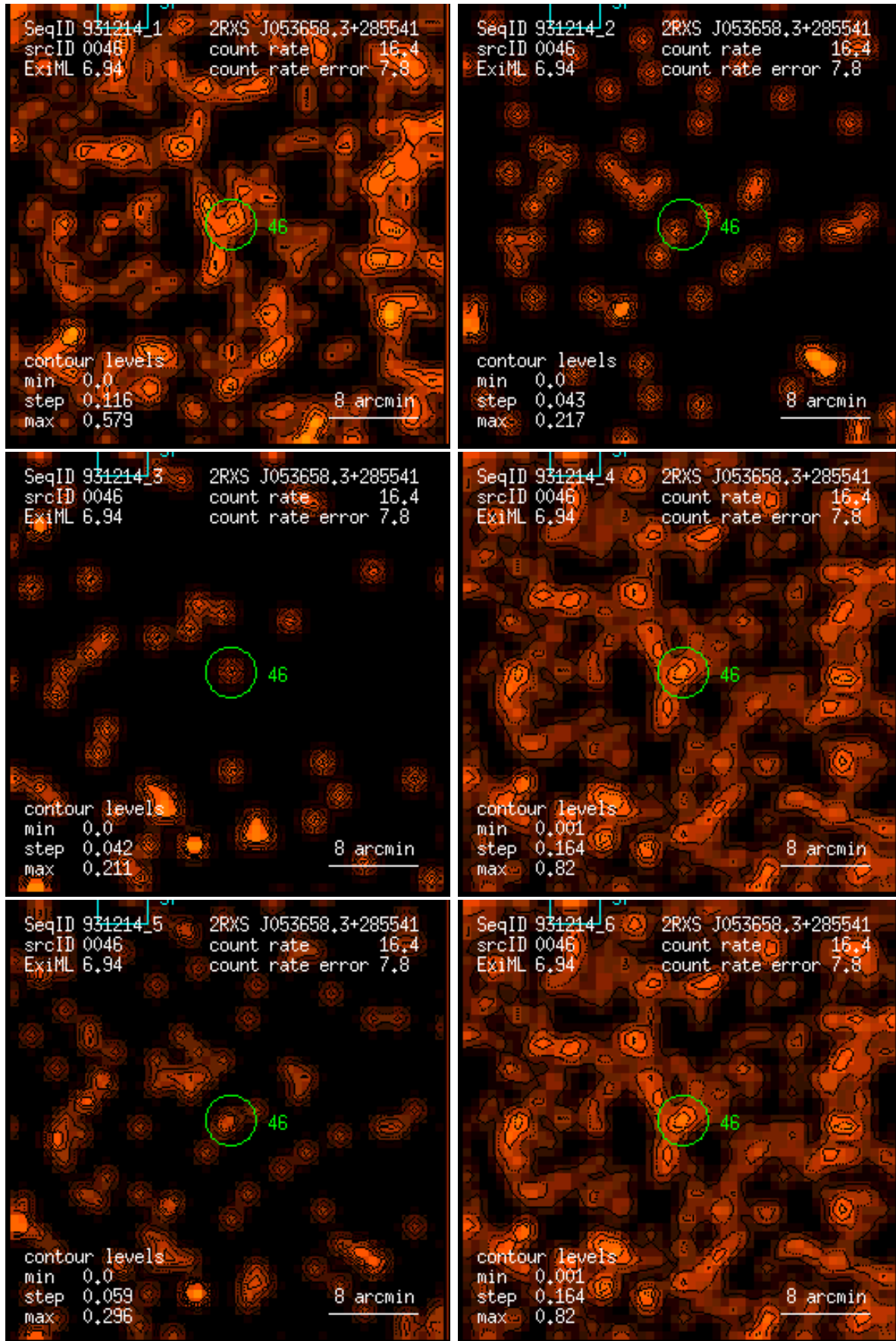
Figure 46: RASS 931214: detection 0046: band rate images, Gaussian filter: (1) PSPC channels 11 – 41, (2) 52 – 90, (3) 91 – 201, (4) 11 – 235, (5) 52 – 201, (6) 11 – 201. Broad band rates in counts/ks. Band rate contour levels in counts/ks/arcmin 2 .
