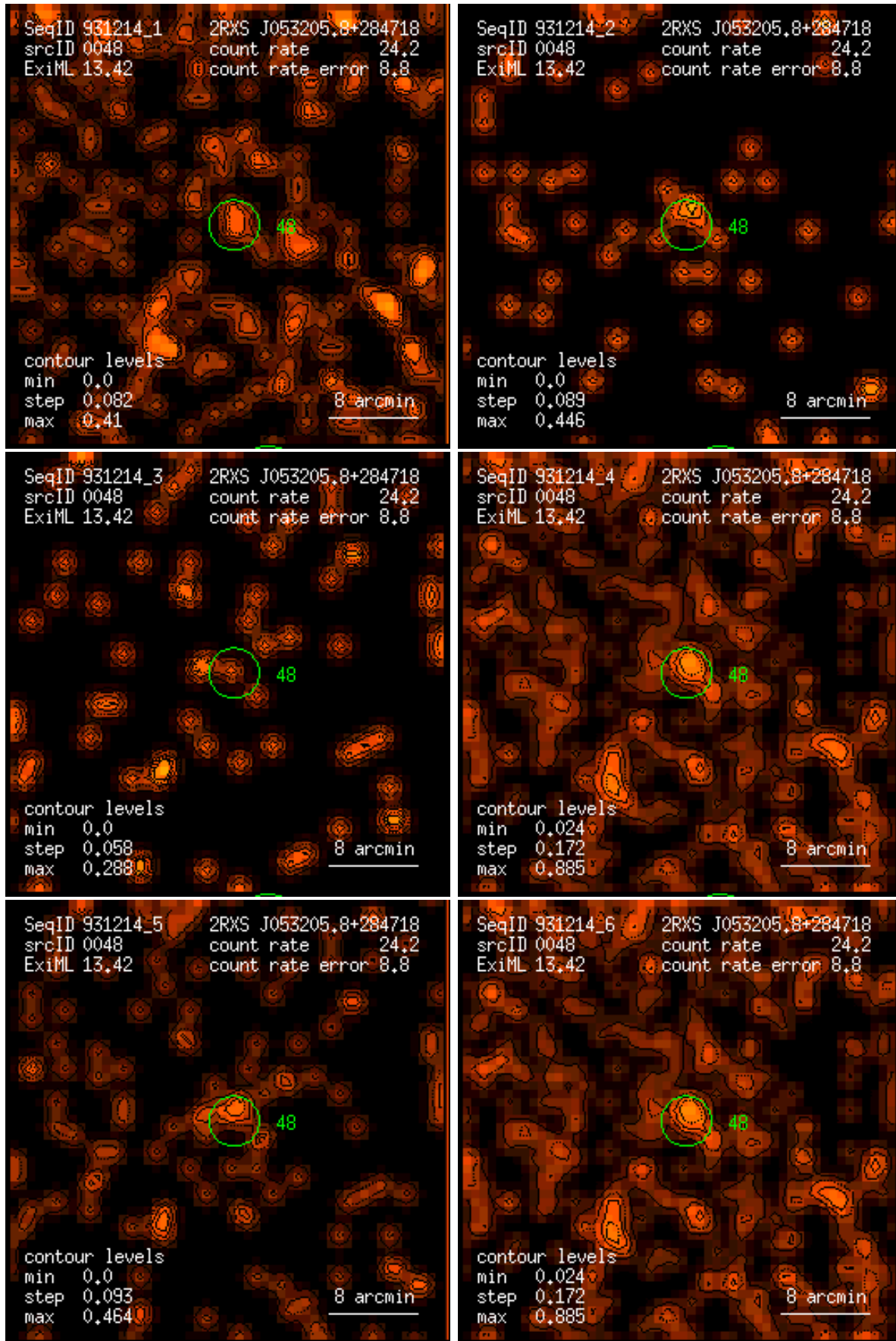
Figure 48: RASS 931214: detection 0048: band rate images, Gaussian filter: (1) PSPC channels 11 – 41, (2) 52 – 90, (3) 91 – 201, (4) 11 – 235, (5) 52 – 201, (6) 11 – 201. Broad band rates in counts/ks. Band rate contour levels in counts/ks/arcmin 2 .
