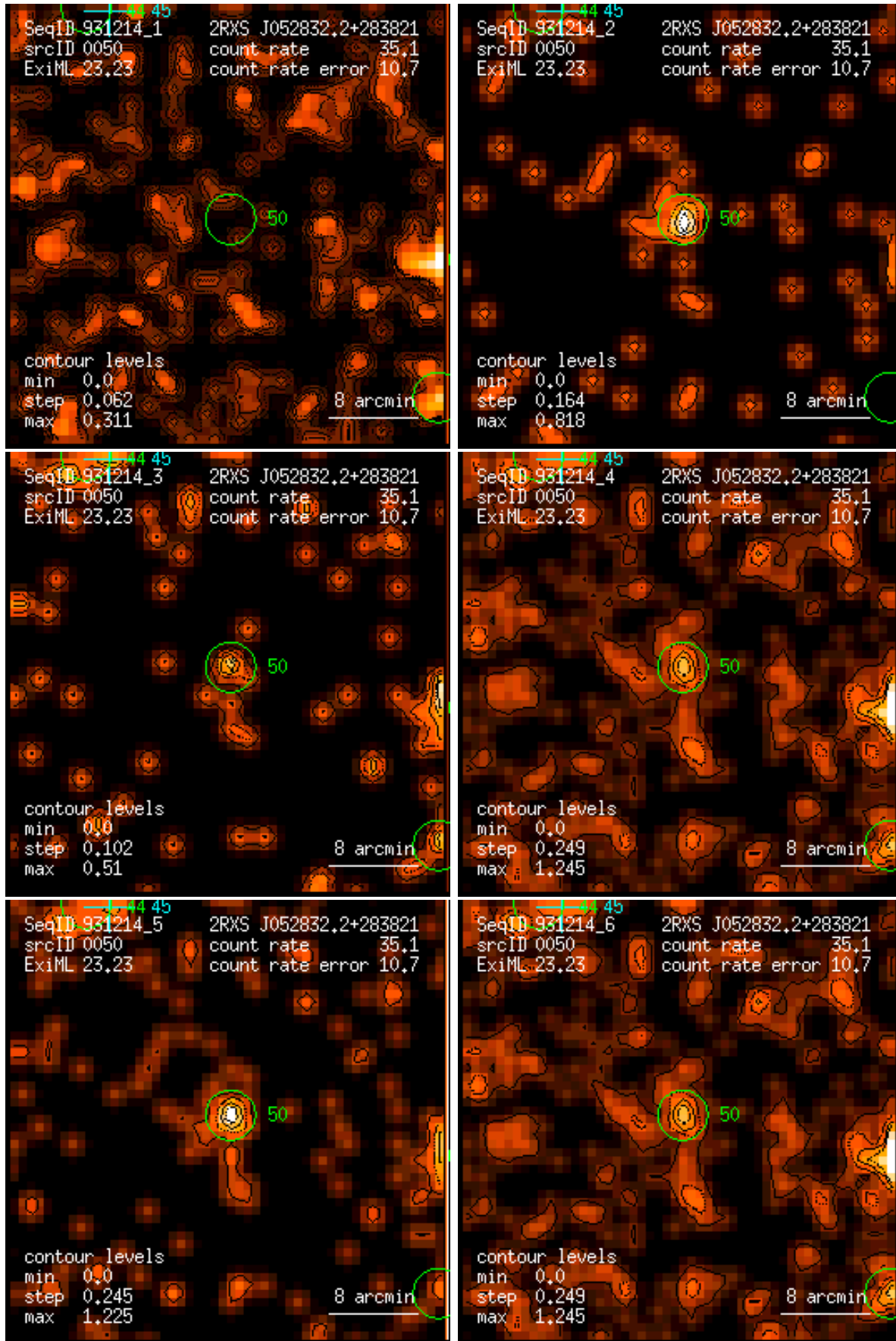
Figure 50: RASS 931214: detection 0050: band rate images, Gaussian filter: (1) PSPC channels 11 – 41, (2) 52 – 90, (3) 91 – 201, (4) 11 – 235, (5) 52 – 201, (6) 11 – 201. Broad band rates in counts/ks. Band rate contour levels in counts/ks/arcmin 2 .
