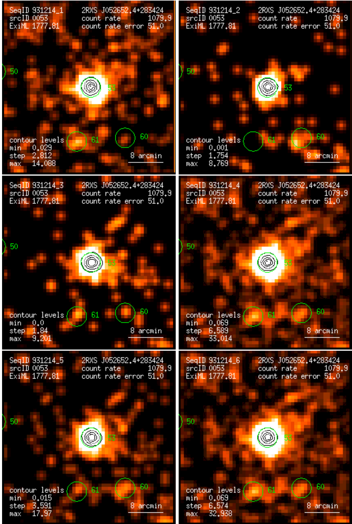
Figure 53: RASS 931214: detection 0053: band rate images, Gaussian filter: (1) PSPC channels 11 – 41, (2) 52 – 90, (3) 91 – 201, (4) 11 – 235, (5) 52 – 201, (6) 11 – 201. Broad band rates in counts/ks. Band rate contour levels in counts/ks/arcmin 2 .
