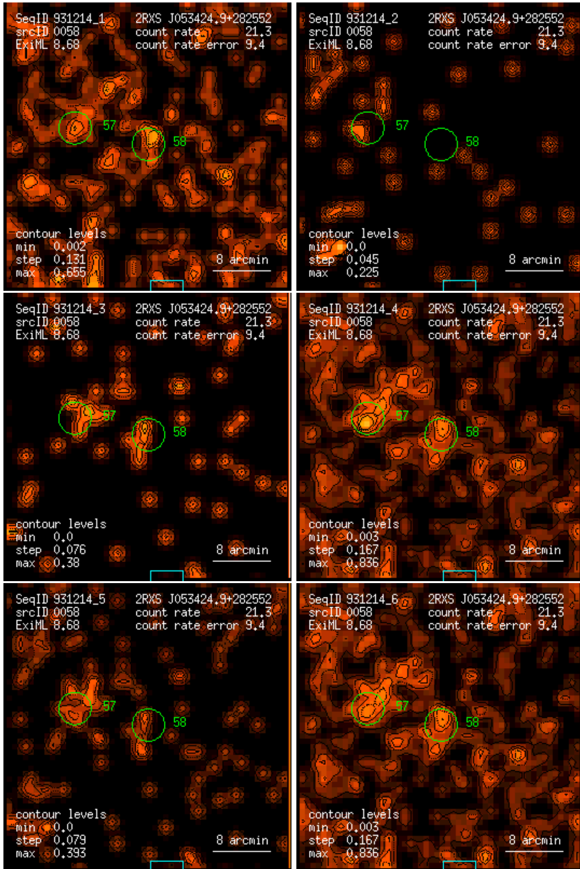
Figure 58: RASS 931214: detection 0058: band rate images, Gaussian filter: (1) PSPC channels 11 – 41, (2) 52 – 90, (3) 91 – 201, (4) 11 – 235, (5) 52 – 201, (6) 11 – 201. Broad band rates in counts/ks. Band rate contour levels in counts/ks/arcmin 2 .
