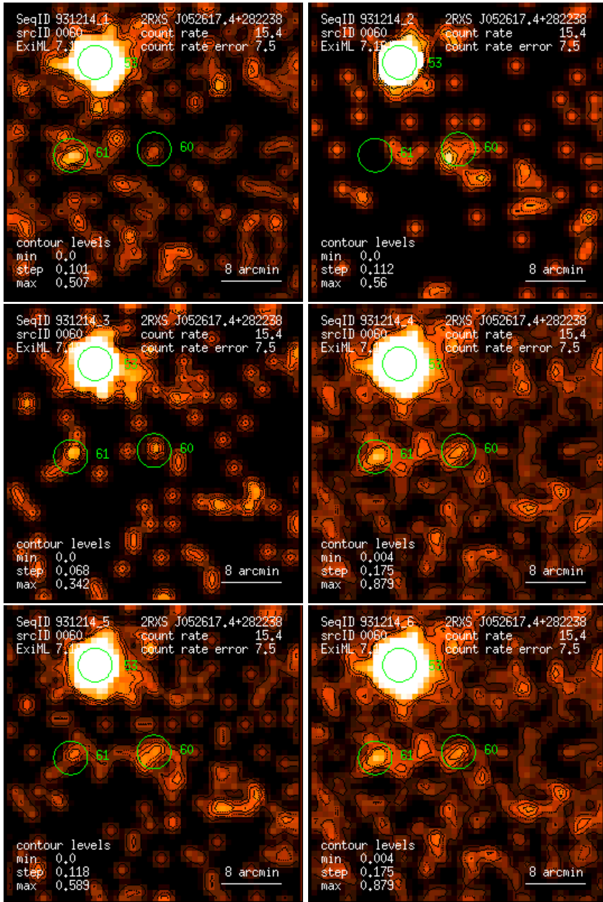
Figure 60: RASS 931214: detection 0060: band rate images, Gaussian filter: (1) PSPC channels 11 – 41, (2) 52 – 90, (3) 91 – 201, (4) 11 – 235, (5) 52 – 201, (6) 11 – 201. Broad band rates in counts/ks. Band rate contour levels in counts/ks/arcmin 2 .
