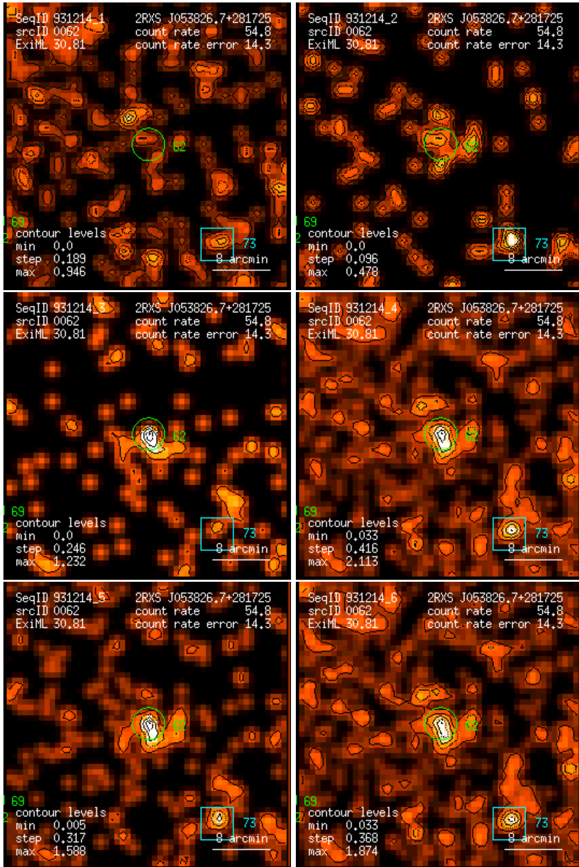
Figure 62: RASS 931214: detection 0062: band rate images, Gaussian filter: (1) PSPC channels 11 – 41, (2) 52 – 90, (3) 91 – 201, (4) 11 – 235, (5) 52 – 201, (6) 11 – 201. Broad band rates in counts/ks. Band rate contour levels in counts/ks/arcmin 2 .
