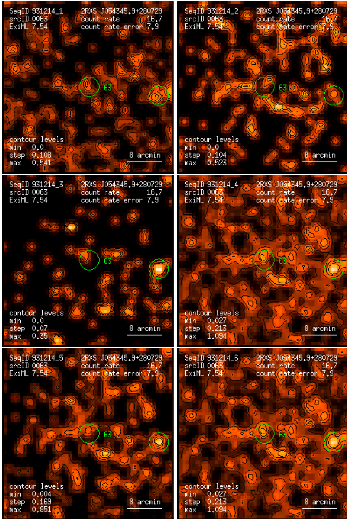
Figure 63: RASS 931214: detection 0063: band rate images, Gaussian filter: (1) PSPC channels 11 – 41, (2) 52 – 90, (3) 91 – 201, (4) 11 – 235, (5) 52 – 201, (6) 11 – 201. Broad band rates in counts/ks. Band rate contour levels in counts/ks/arcmin 2 .
