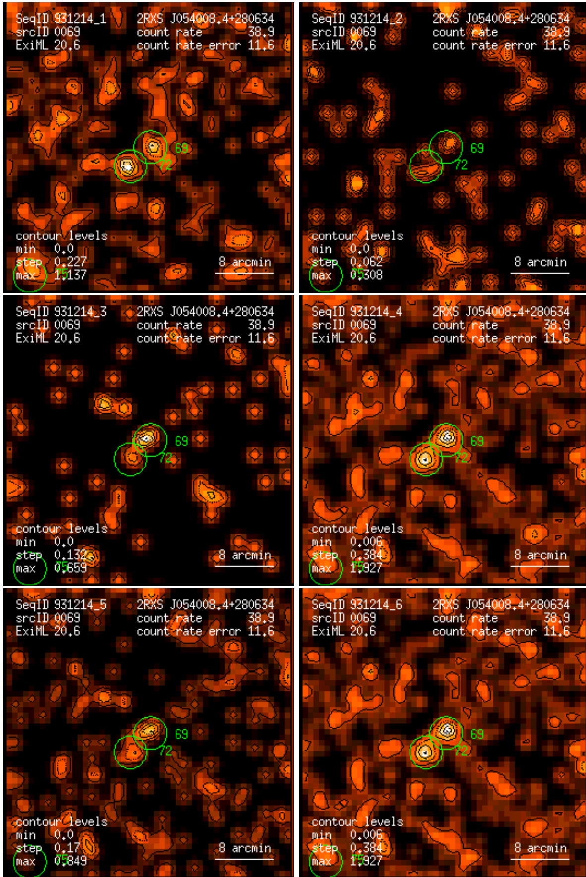
Figure 69: RASS 931214: detection 0069: band rate images, Gaussian filter: (1) PSPC channels 11 – 41, (2) 52 – 90, (3) 91 – 201, (4) 11 – 235, (5) 52 – 201, (6) 11 – 201. Broad band rates in counts/ks. Band rate contour levels in counts/ks/arcmin 2 .
