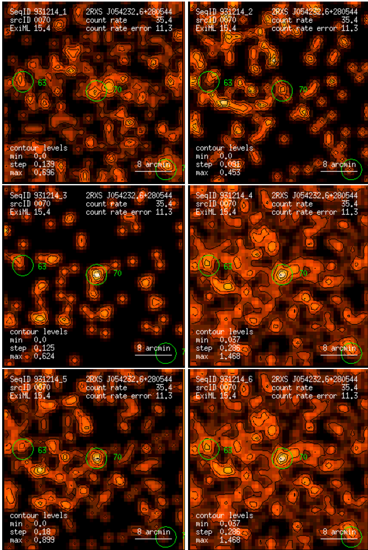
Figure 70: RASS 931214: detection 0070: band rate images, Gaussian filter: (1) PSPC channels 11 – 41, (2) 52 – 90, (3) 91 – 201, (4) 11 – 235, (5) 52 – 201, (6) 11 – 201. Broad band rates in counts/ks. Band rate contour levels in counts/ks/arcmin 2 .
