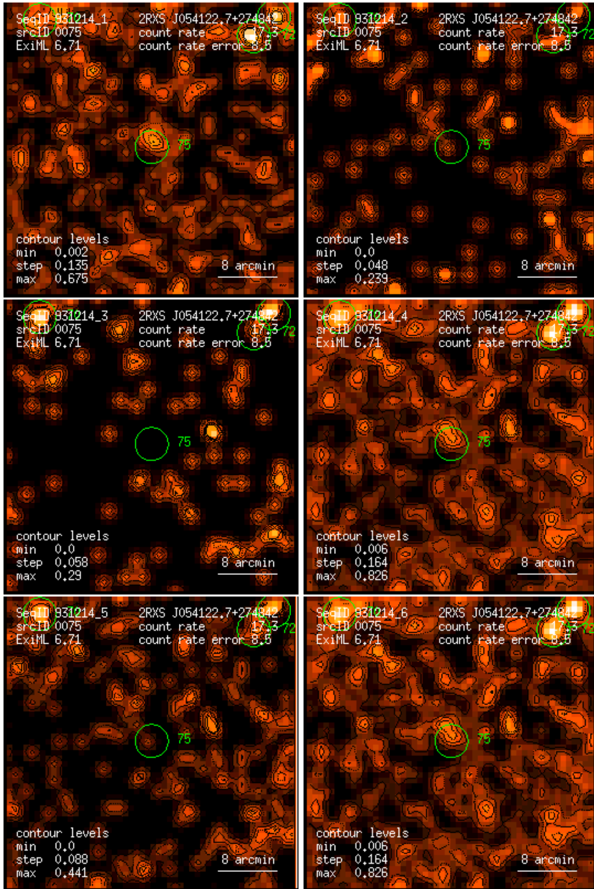
Figure 75: RASS 931214: detection 0075: band rate images, Gaussian filter: (1) PSPC channels 11 – 41, (2) 52 – 90, (3) 91 – 201, (4) 11 – 235, (5) 52 – 201, (6) 11 – 201. Broad band rates in counts/ks. Band rate contour levels in counts/ks/arcmin 2 .
