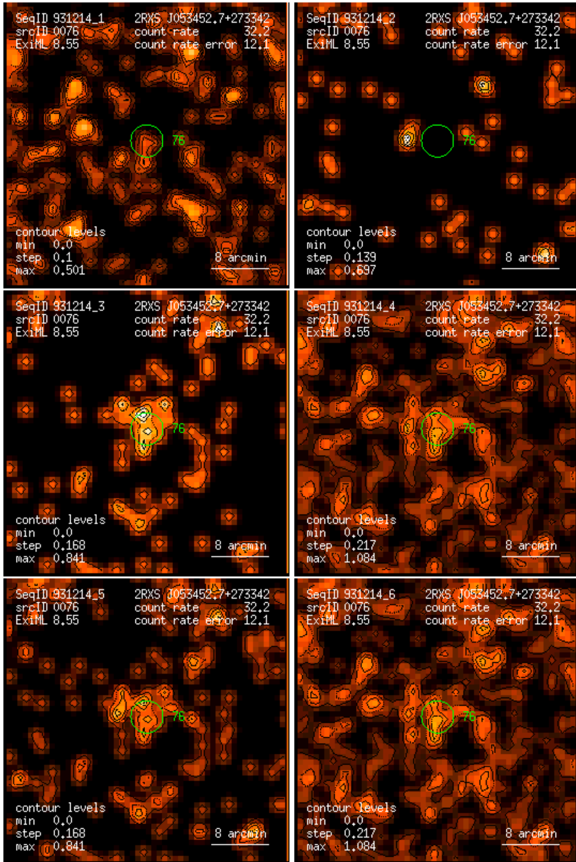
Figure 76: RASS 931214: detection 0076: band rate images, Gaussian filter: (1) PSPC channels 11 – 41, (2) 52 – 90, (3) 91 – 201, (4) 11 – 235, (5) 52 – 201, (6) 11 – 201. Broad band rates in counts/ks. Band rate contour levels in counts/ks/arcmin 2 .
