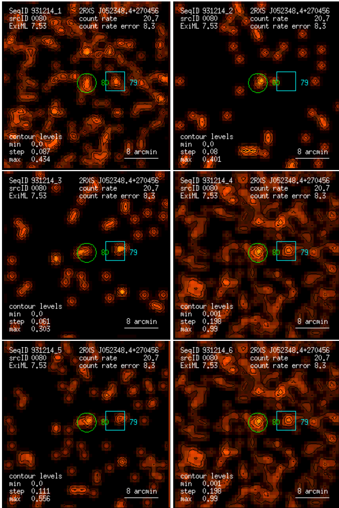
Figure 80: RASS 931214: detection 0080: band rate images, Gaussian filter: (1) PSPC channels 11 – 41, (2) 52 – 90, (3) 91 – 201, (4) 11 – 235, (5) 52 – 201, (6) 11 – 201. Broad band rates in counts/ks. Band rate contour levels in counts/ks/arcmin 2 .
