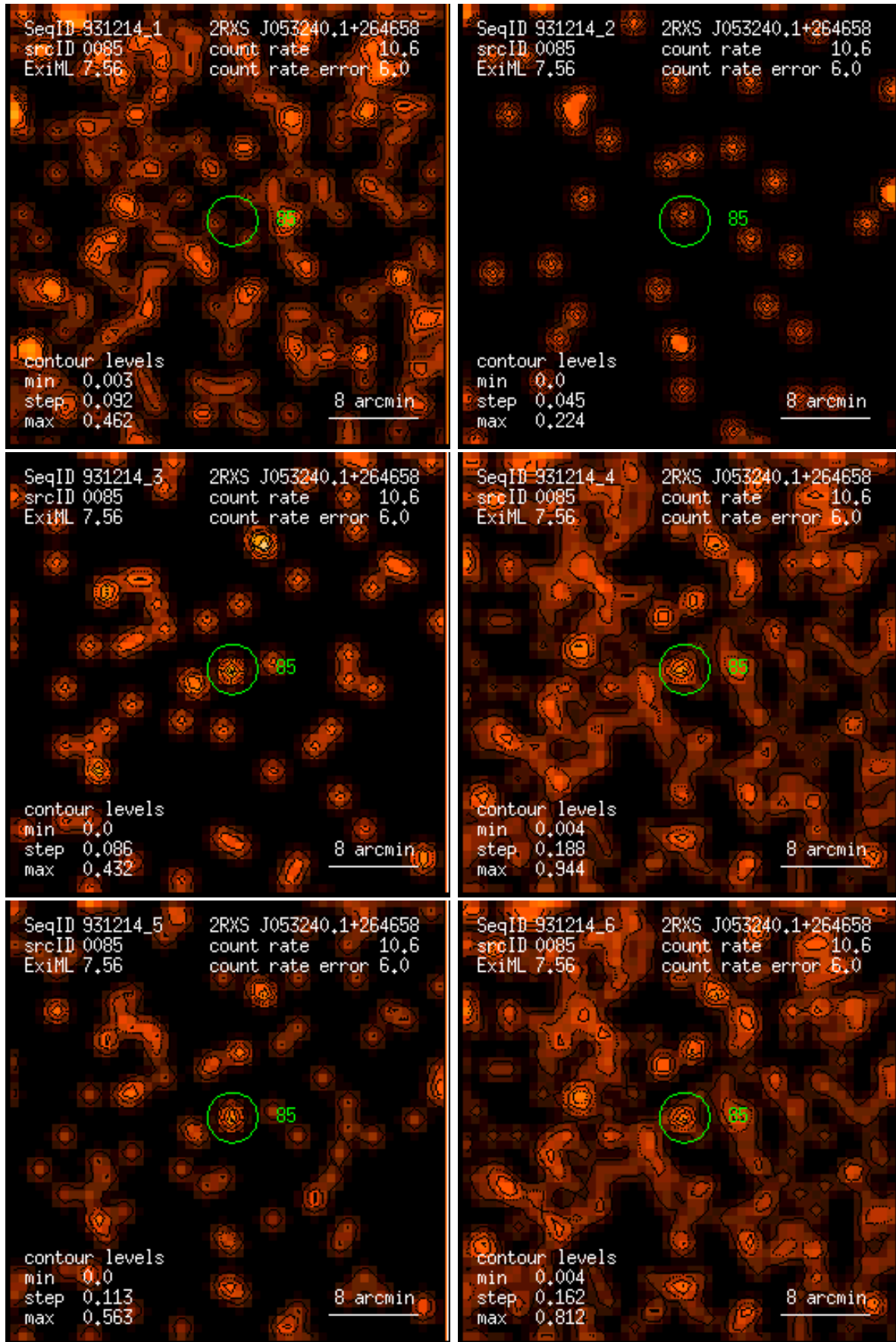
Figure 85: RASS 931214: detection 0085: band rate images, Gaussian filter: (1) PSPC channels 11 – 41, (2) 52 – 90, (3) 91 – 201, (4) 11 – 235, (5) 52 – 201, (6) 11 – 201. Broad band rates in counts/ks. Band rate contour levels in counts/ks/arcmin 2 .
