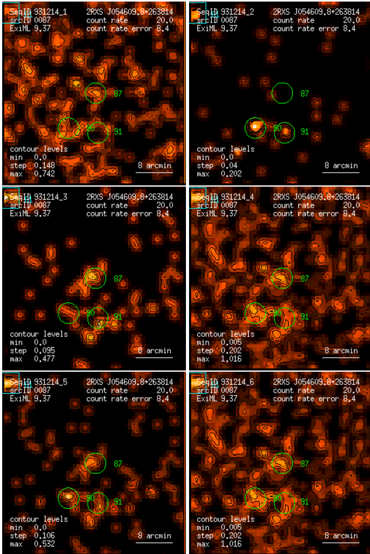
Figure 87: RASS 931214: detection 0087: band rate images, Gaussian filter: (1) PSPC channels 11 – 41, (2) 52 – 90, (3) 91 – 201, (4) 11 – 235, (5) 52 – 201, (6) 11 – 201. Broad band rates in counts/ks. Band rate contour levels in counts/ks/arcmin 2 .
