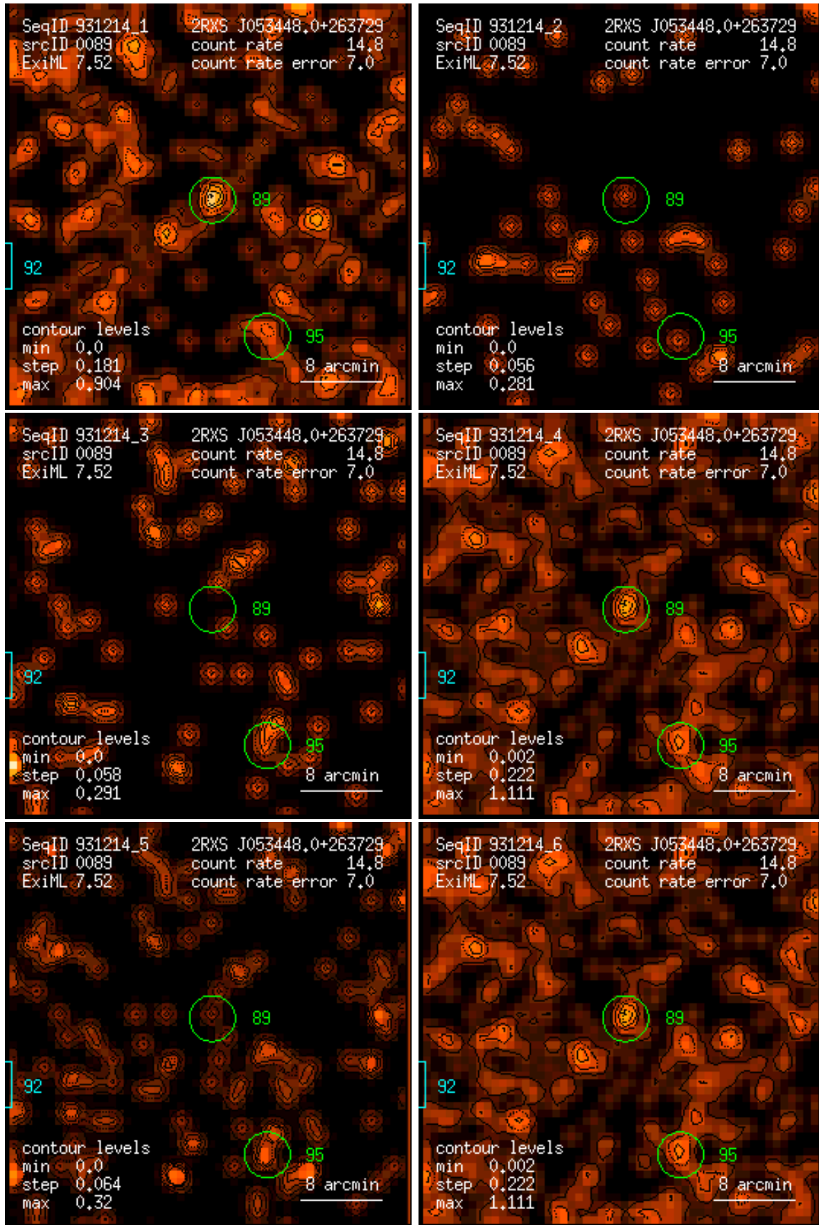
Figure 89: RASS 931214: detection 0089: band rate images, Gaussian filter: (1) PSPC channels 11 – 41, (2) 52 – 90, (3) 91 – 201, (4) 11 – 235, (5) 52 – 201, (6) 11 – 201. Broad band rates in counts/ks. Band rate contour levels in counts/ks/arcmin 2 .
