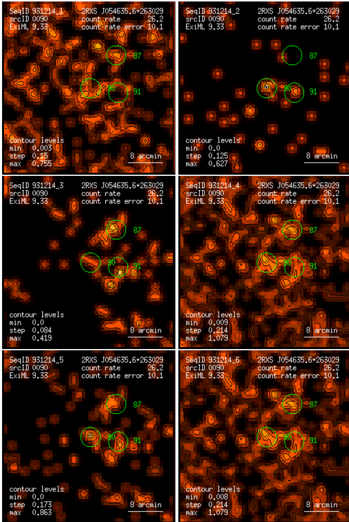
Figure 90: RASS 931214: detection 0090: band rate images, Gaussian filter: (1) PSPC channels 11 – 41, (2) 52 – 90, (3) 91 – 201, (4) 11 – 235, (5) 52 – 201, (6) 11 – 201. Broad band rates in counts/ks. Band rate contour levels in counts/ks/arcmin 2 .
