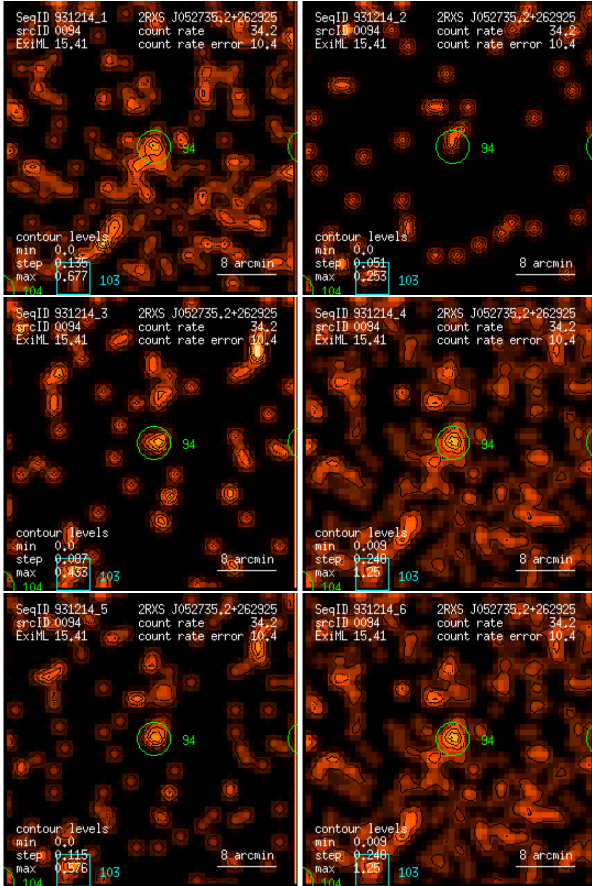
Figure 94: RASS 931214: detection 0094: band rate images, Gaussian filter: (1) PSPC channels 11 – 41, (2) 52 – 90, (3) 91 – 201, (4) 11 – 235, (5) 52 – 201, (6) 11 – 201. Broad band rates in counts/ks. Band rate contour levels in counts/ks/arcmin 2 .
