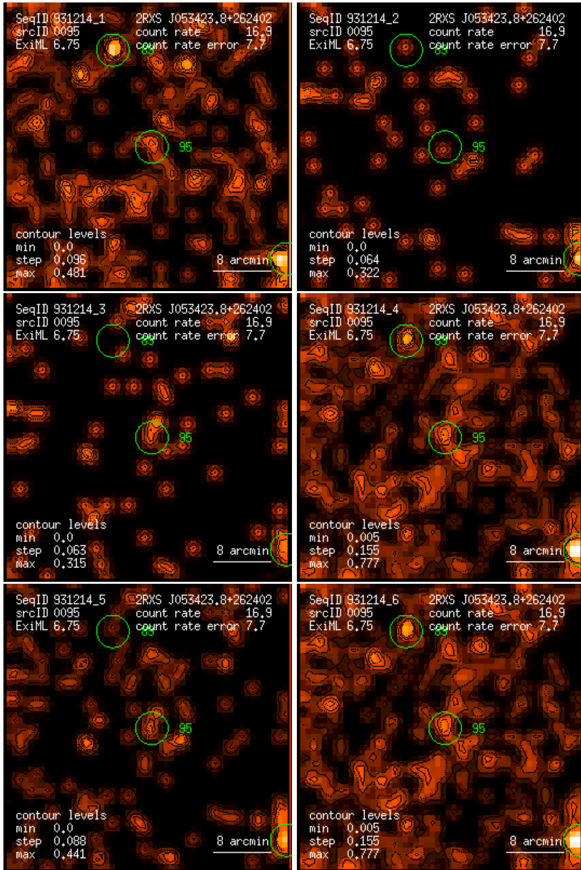
Figure 95: RASS 931214: detection 0095: band rate images, Gaussian filter: (1) PSPC channels 11 – 41, (2) 52 – 90, (3) 91 – 201, (4) 11 – 235, (5) 52 – 201, (6) 11 – 201. Broad band rates in counts/ks. Band rate contour levels in counts/ks/arcmin 2 .
