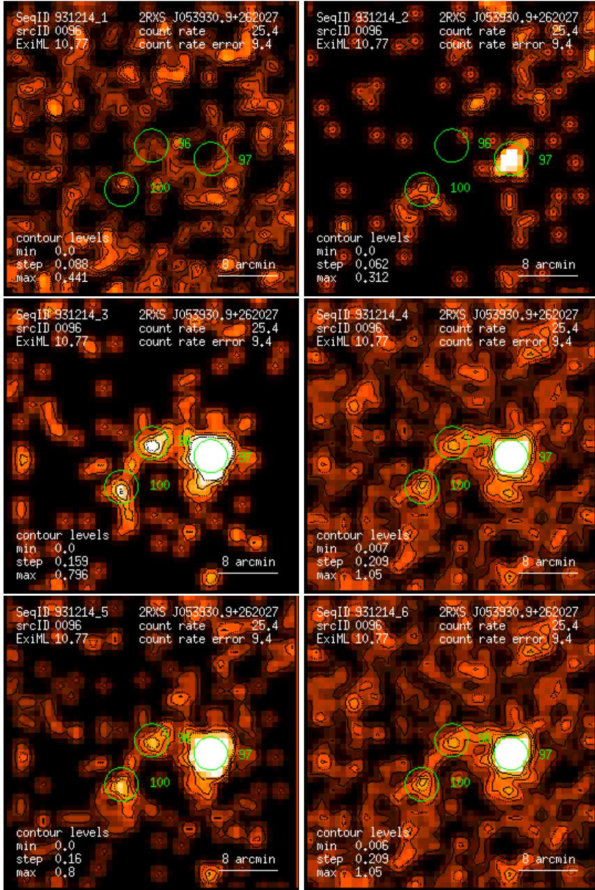
Figure 96: RASS 931214: detection 0096: band rate images, Gaussian filter: (1) PSPC channels 11 – 41, (2) 52 – 90, (3) 91 – 201, (4) 11 – 235, (5) 52 – 201, (6) 11 – 201. Broad band rates in counts/ks. Band rate contour levels in counts/ks/arcmin 2 .
