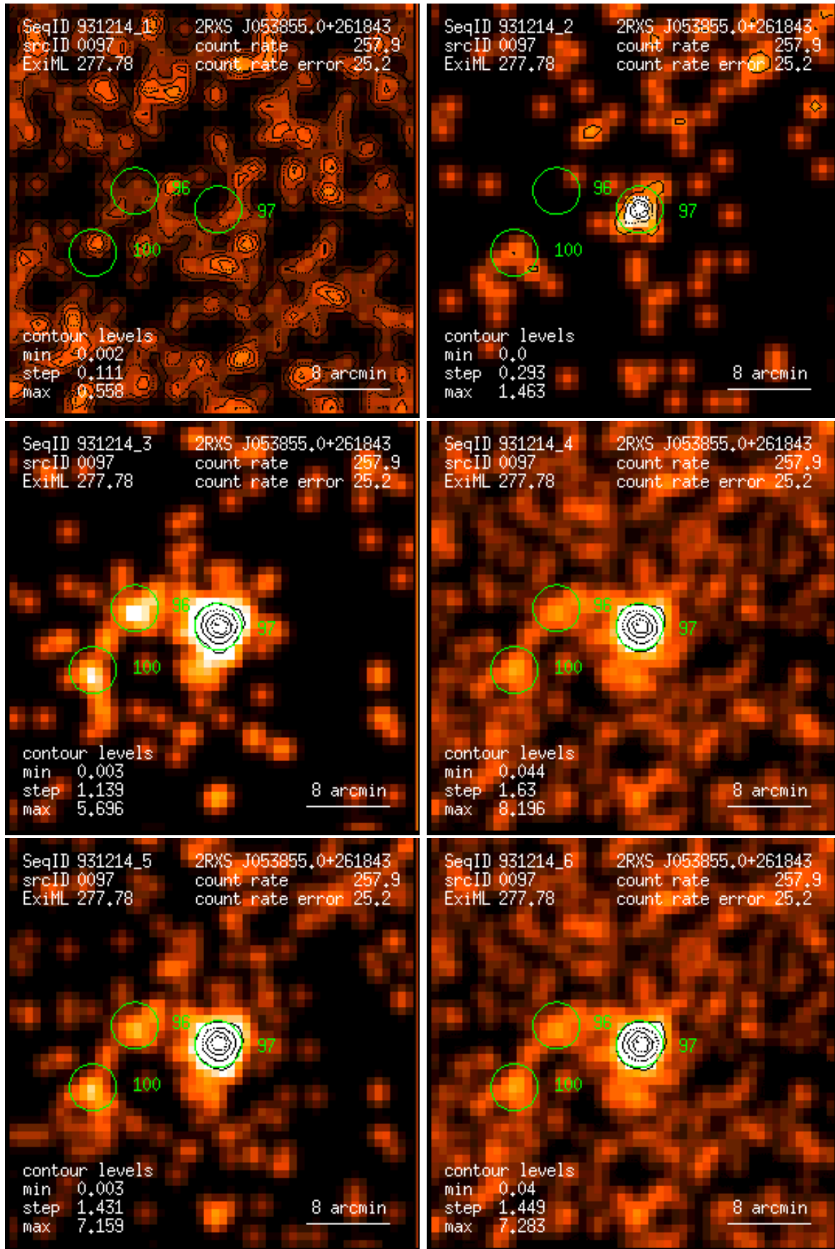
Figure 97: RASS 931214: detection 0097: band rate images, Gaussian filter: (1) PSPC channels 11 – 41, (2) 52 – 90, (3) 91 – 201, (4) 11 – 235, (5) 52 – 201, (6) 11 – 201. Broad band rates in counts/ks. Band rate contour levels in counts/ks/arcmin 2 .
