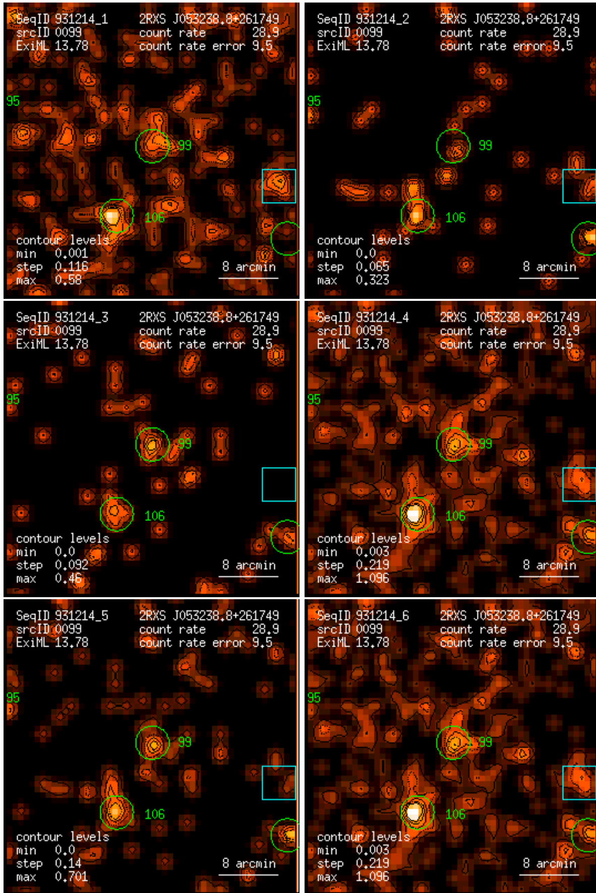
Figure 99: RASS 931214: detection 0099: band rate images, Gaussian filter: (1) PSPC channels 11 – 41, (2) 52 – 90, (3) 91 – 201, (4) 11 – 235, (5) 52 – 201, (6) 11 – 201. Broad band rates in counts/ks. Band rate contour levels in counts/ks/arcmin 2 .
