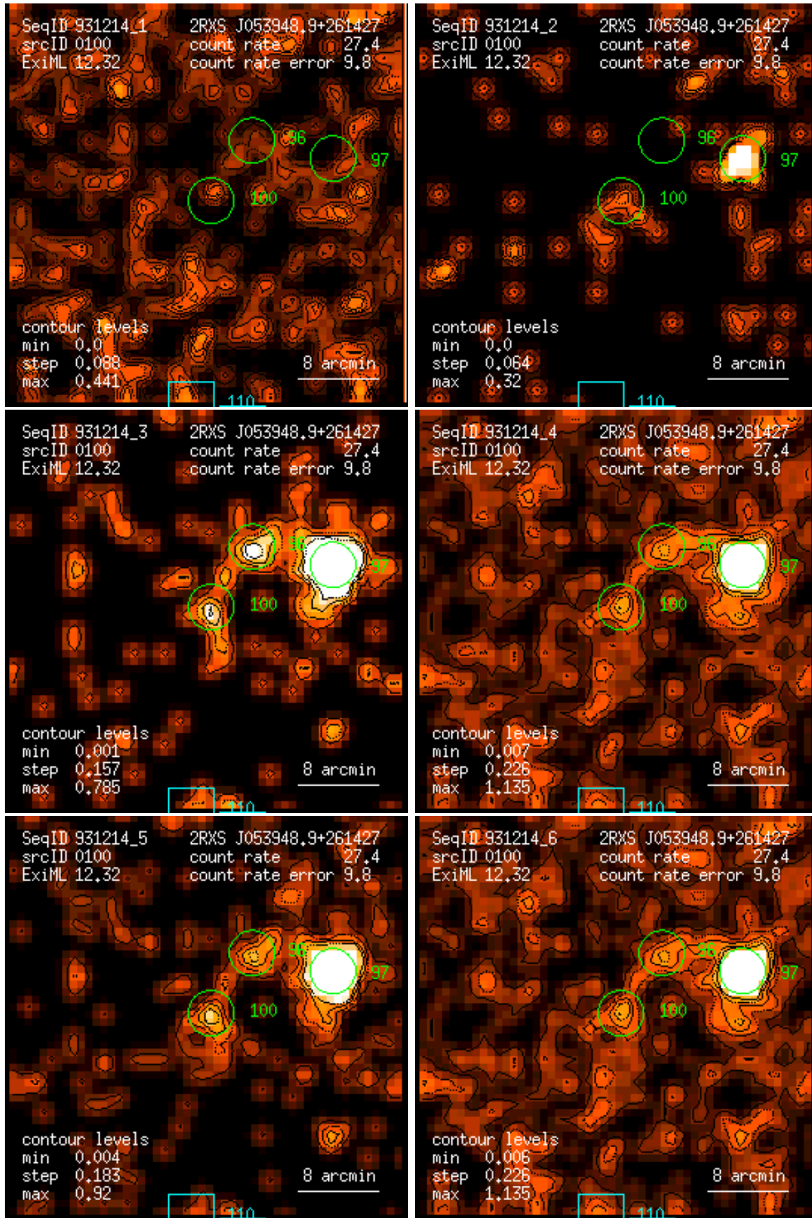
Figure 100: RASS 931214: detection 0100: band rate images, Gaussian filter: (1) PSPC channels 11 – 41, (2) 52 – 90, (3) 91 – 201, (4) 11 – 235, (5) 52 – 201, (6) 11 – 201. Broad band rates in counts/ks. Band rate contour levels in counts/ks/arcmin 2 .
