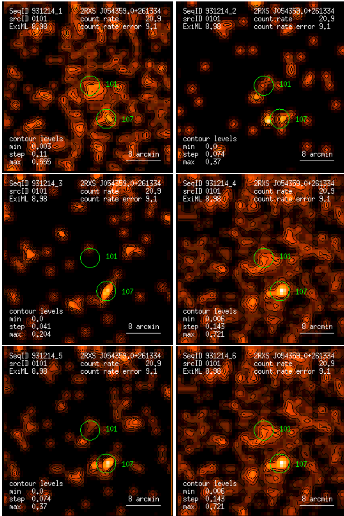
Figure 101: RASS 931214: detection 0101: band rate images, Gaussian filter: (1) PSPC channels 11 – 41, (2) 52 – 90, (3) 91 – 201, (4) 11 – 235, (5) 52 – 201, (6) 11 – 201. Broad band rates in counts/ks. Band rate contour levels in counts/ks/arcmin 2 .
